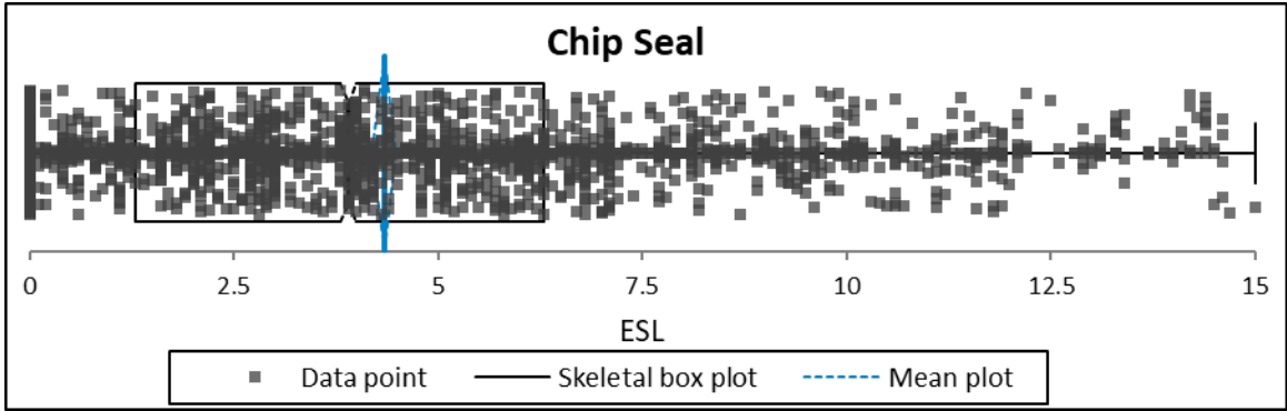
Figure 10: Chip seal non-weighted average ESL segment distribution
